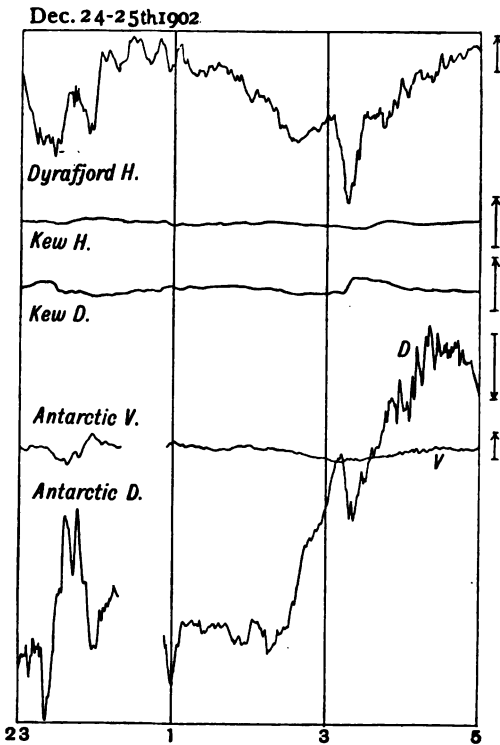
FIG. 35.—ARCTIC-KEW-ANTARCTIC CURVES.
